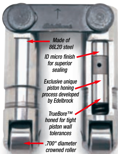
Cutaway of Hydraulic Roller Lifter
